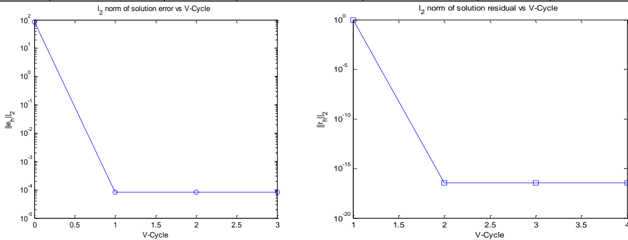
Figure 4.1: Left side figure shows the error graph and right side figure shows graph of the residuals norm. N=127 are the number of nodes.
